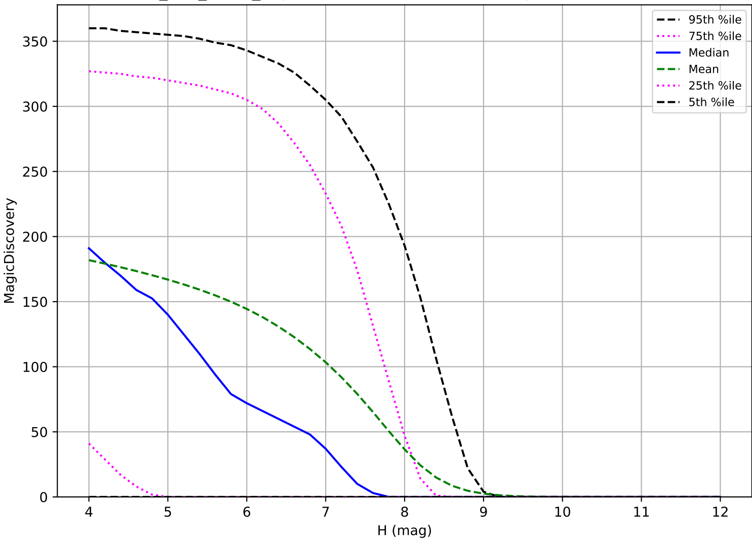
too_100_1v3.4_10yrs: TNO 6 detections in 60 nights detection loss
