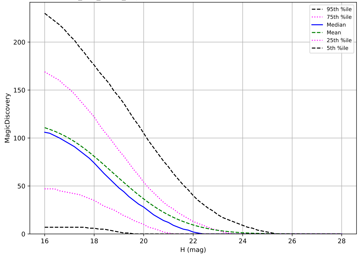
too_100_1v3.4_10yrs: PHA 6 detections in 60 nights detection loss
