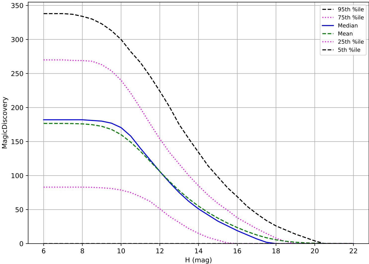
too_100_1v3.4_10yrs: OCC_r5 6 detections in 60 nights detection loss
