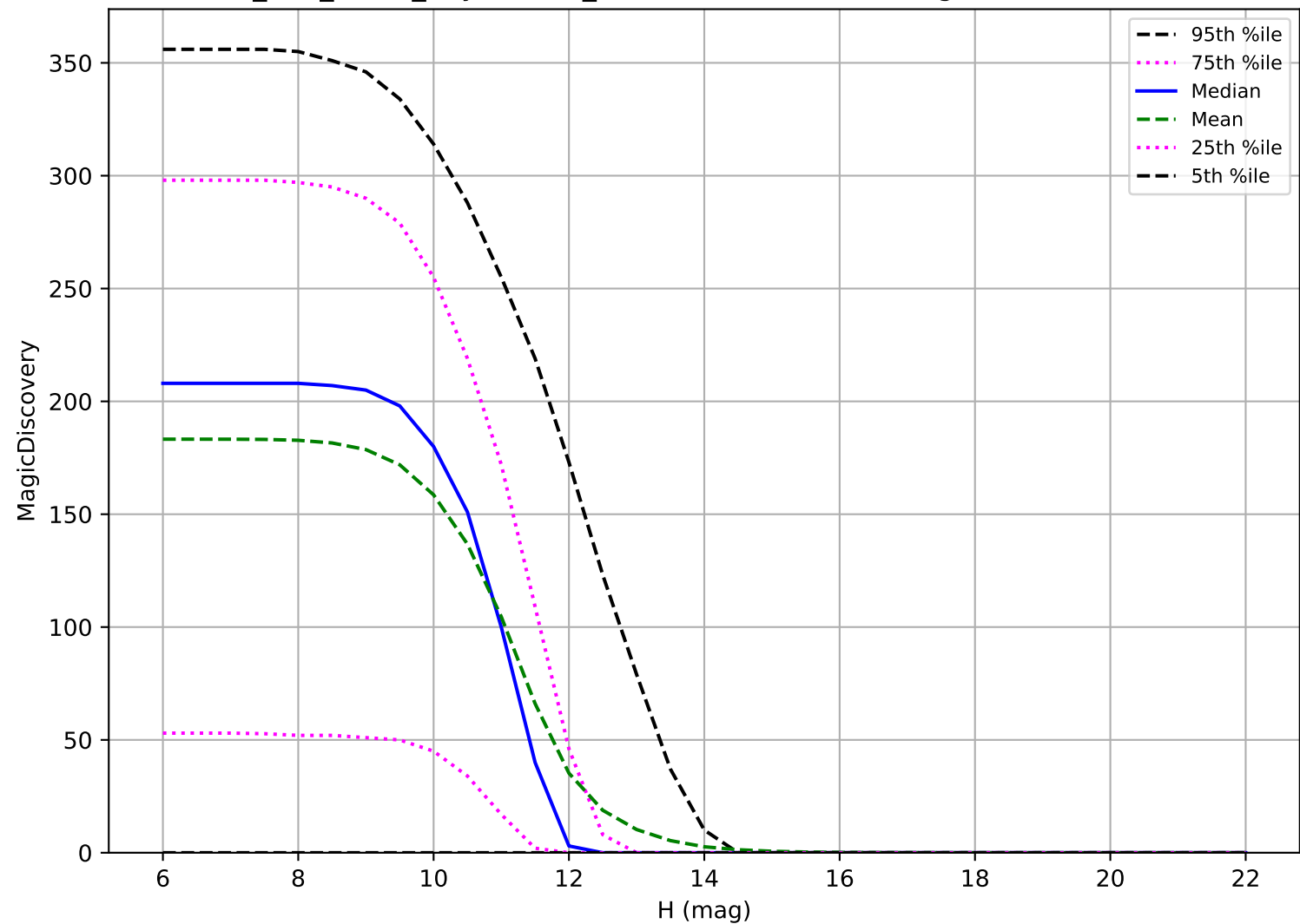
too_100_1v3.4_10yrs: OCC_r20 6 detections in 60 nights detection loss
