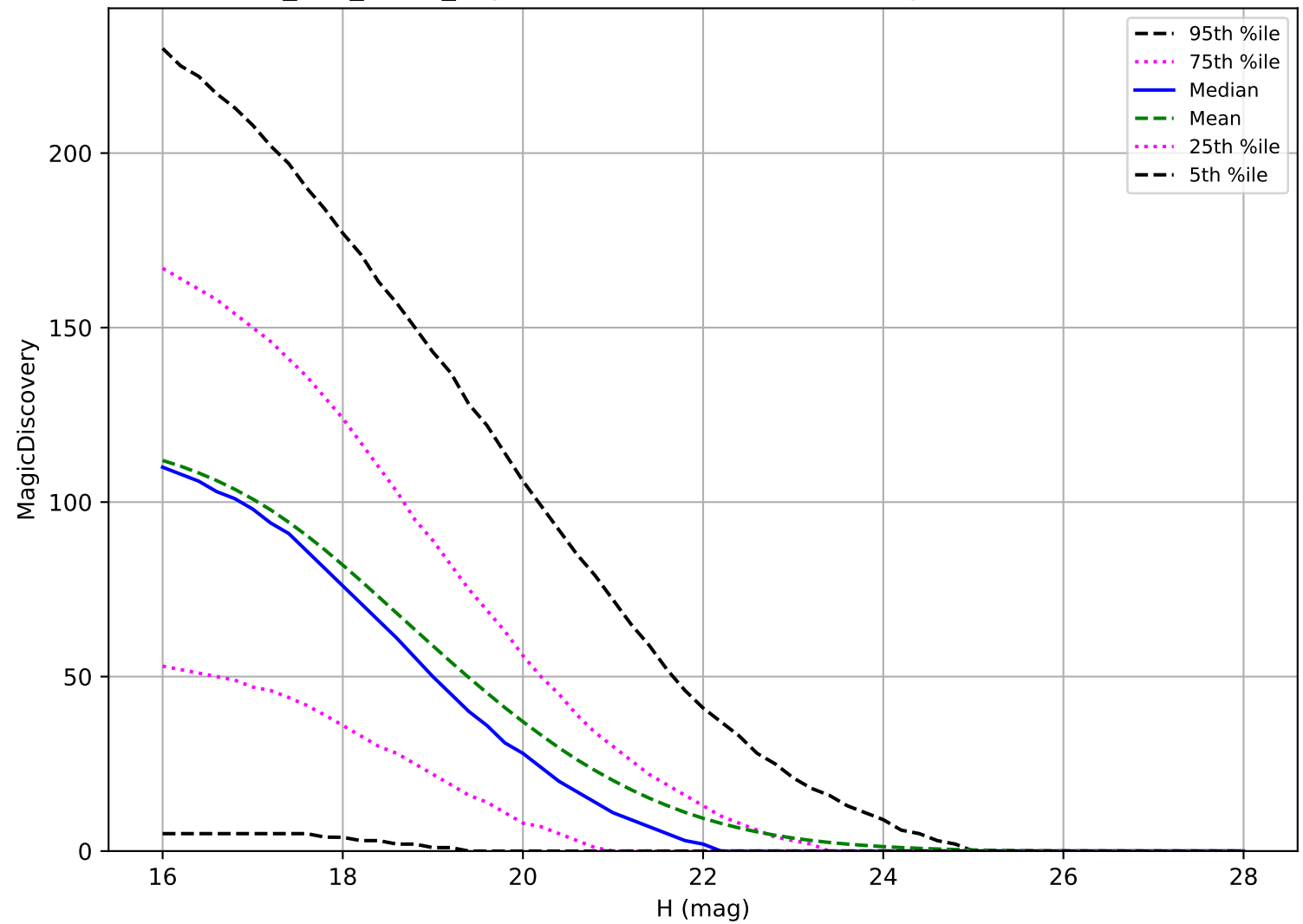
too_100_1v3.4_10yrs: NEO 6 detections in 60 nights detection loss
