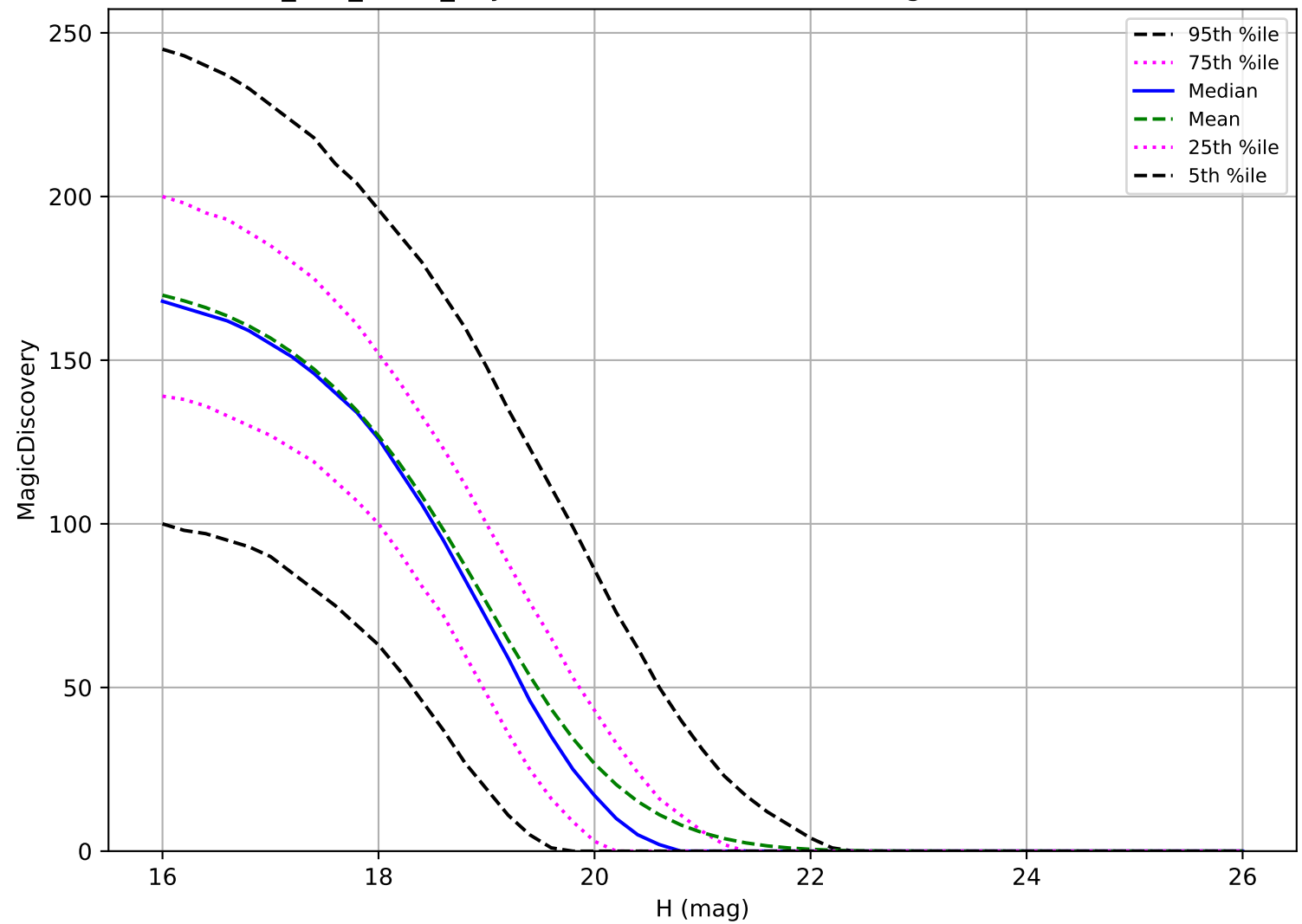
too_100_1v3.4_10yrs: MBA 6 detections in 60 nights detection loss
