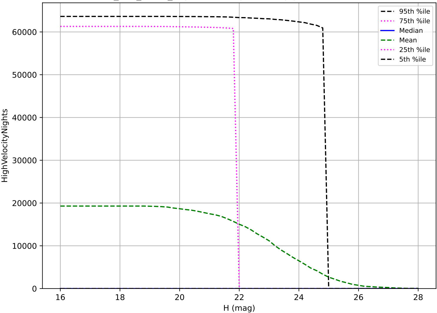
too_100_1v3.4_10yrs: NEO High velocity pair detection loss
