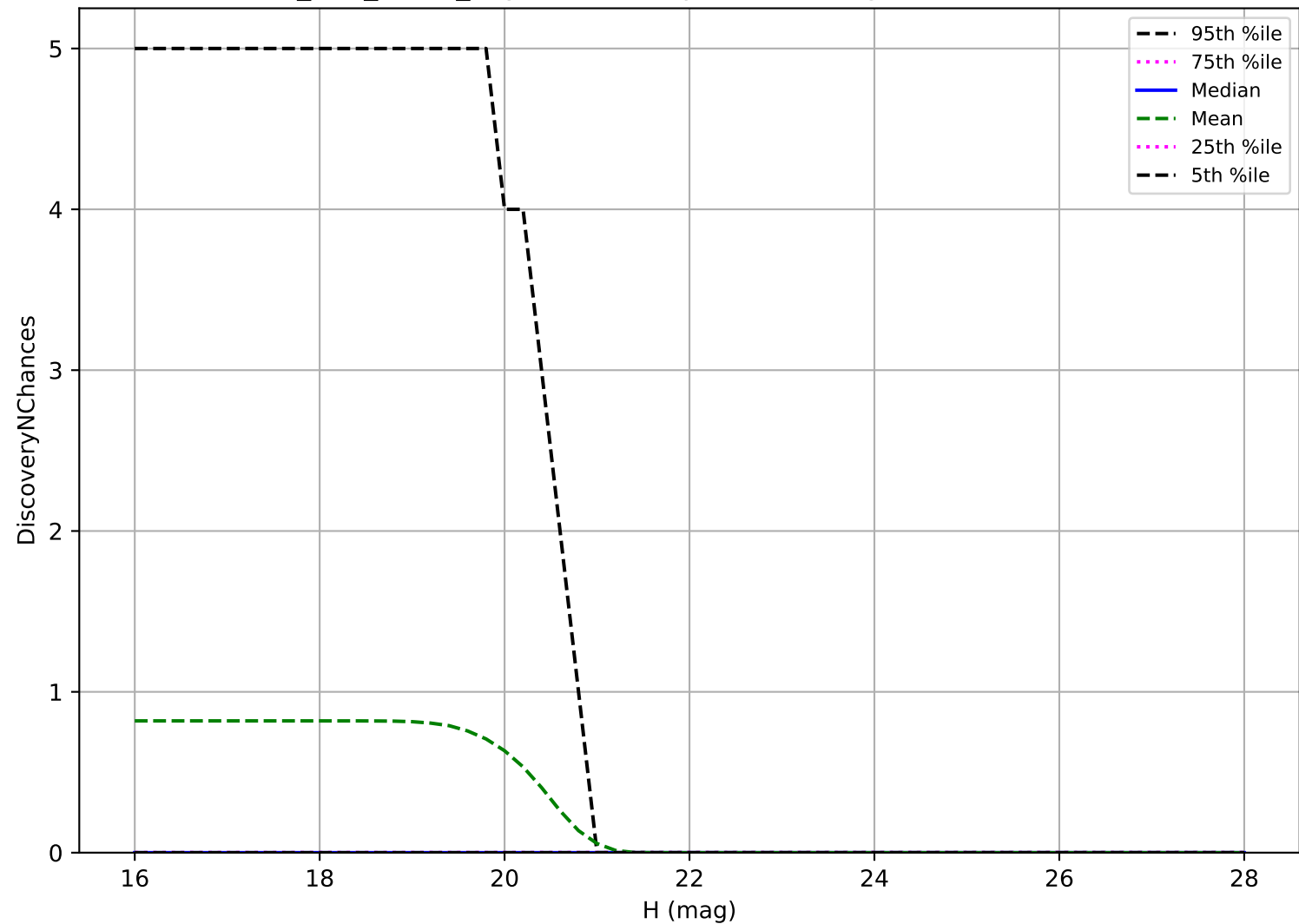
too_100_1v3.4_10yrs: Vatira 3 pairs in 15 nights detection loss
