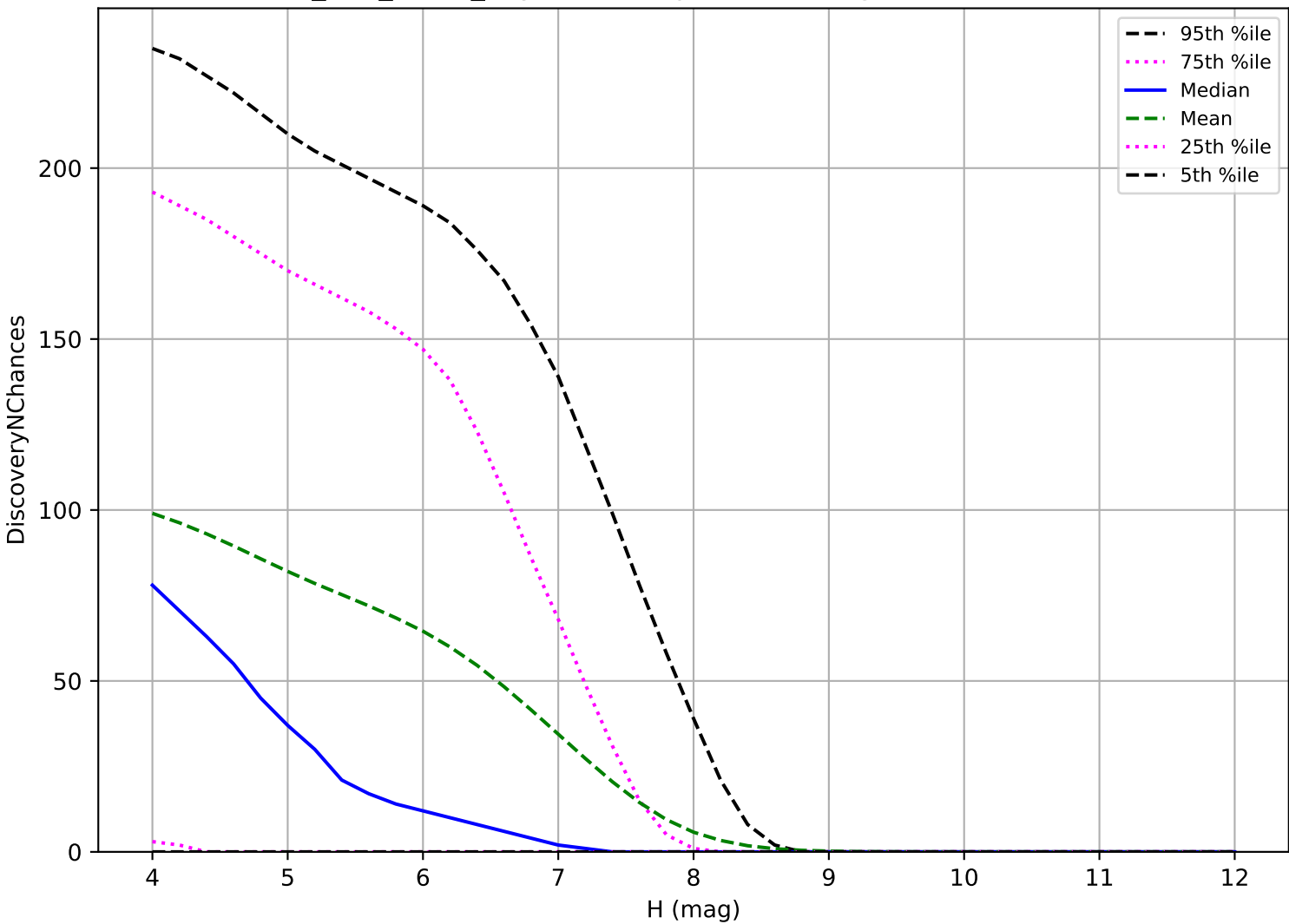
too_100_1v3.4_10yrs: TNO 3 pairs in 15 nights detection loss
