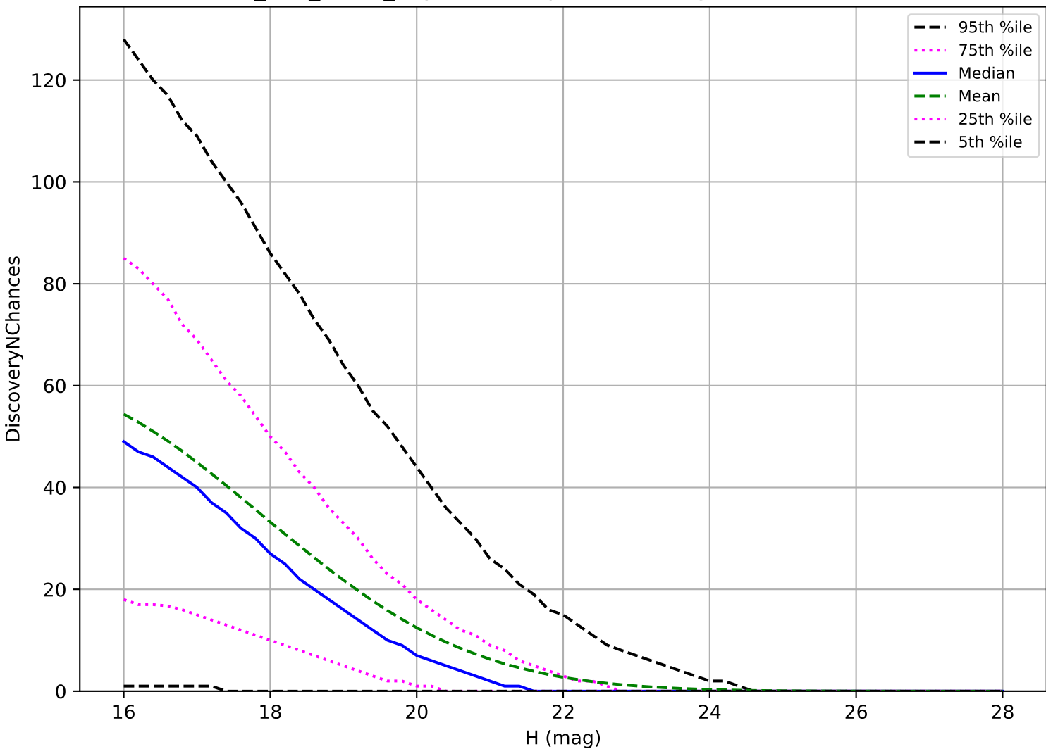
too_100_1v3.4_10yrs: PHA 3 pairs in 15 nights detection loss
