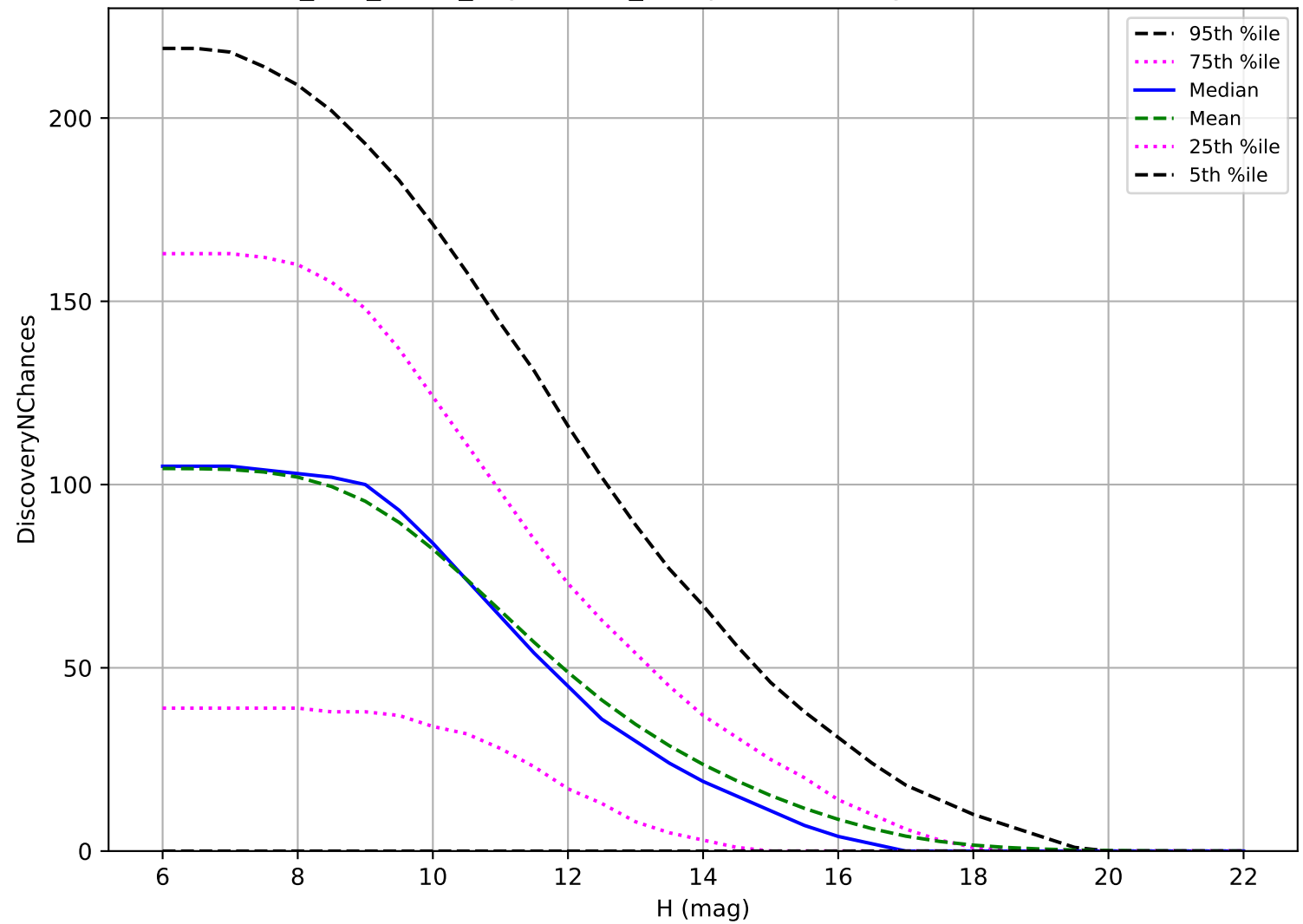
too_100_1v3.4_10yrs: OCC_r5 3 pairs in 15 nights detection loss
