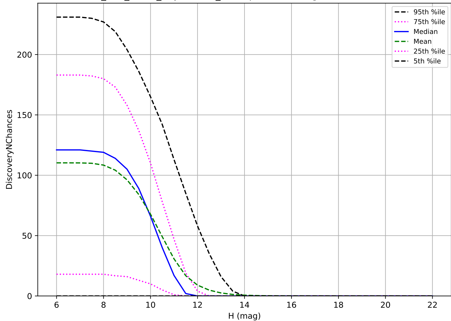
too_100_1v3.4_10yrs: OCC_r20 3 pairs in 15 nights detection loss
