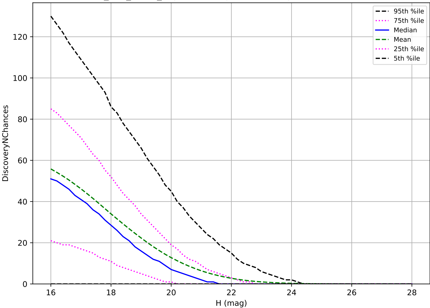
too_100_1v3.4_10yrs: NEO 3 pairs in 15 nights detection loss
