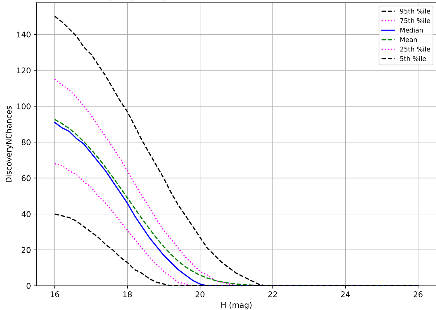
too_100_1v3.4_10yrs: MBA 3 pairs in 15 nights detection loss
