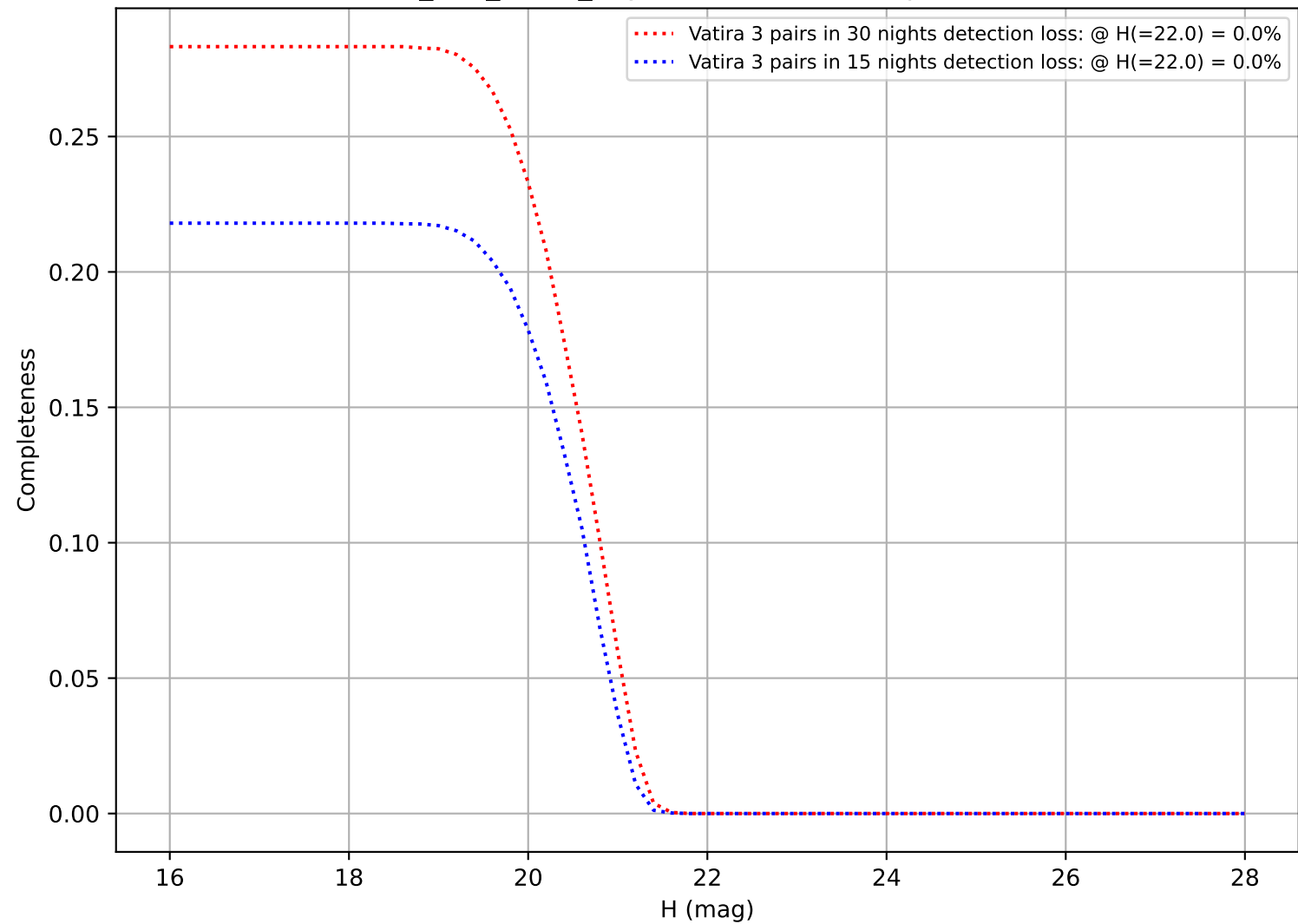
too_100_1v3.4_10yrs: DifferentialCompleteness
