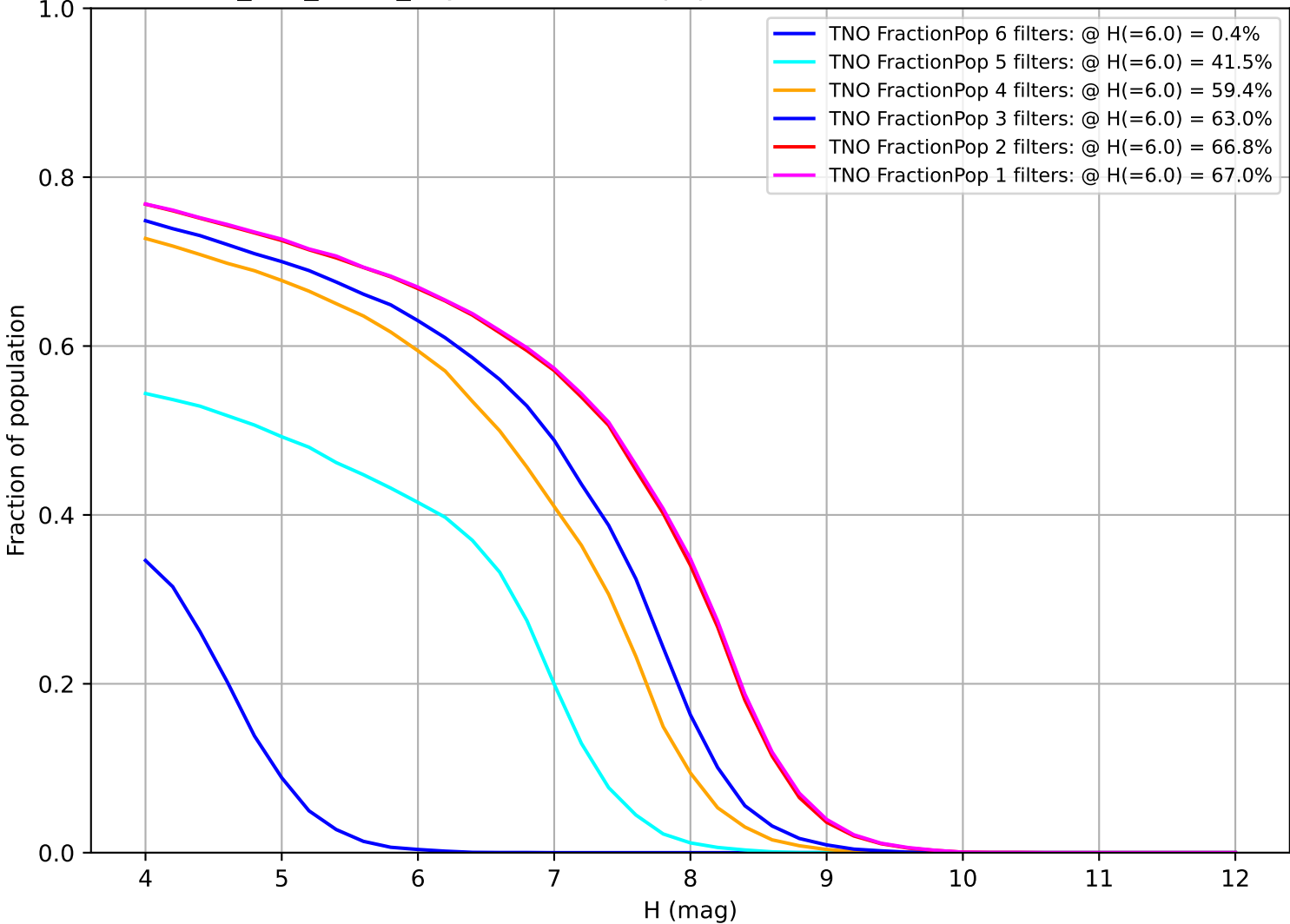
too_100_1v3.4_10yrs: Fraction of population with colors in X filters TNO
