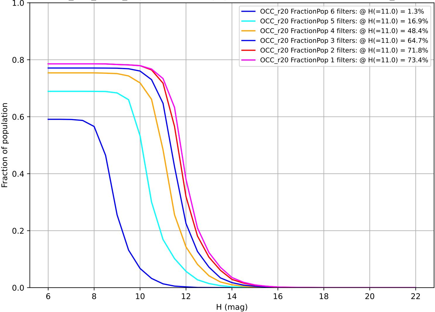
too_100_1v3.4_10yrs: Fraction of population with colors in X filters OCC_r20
