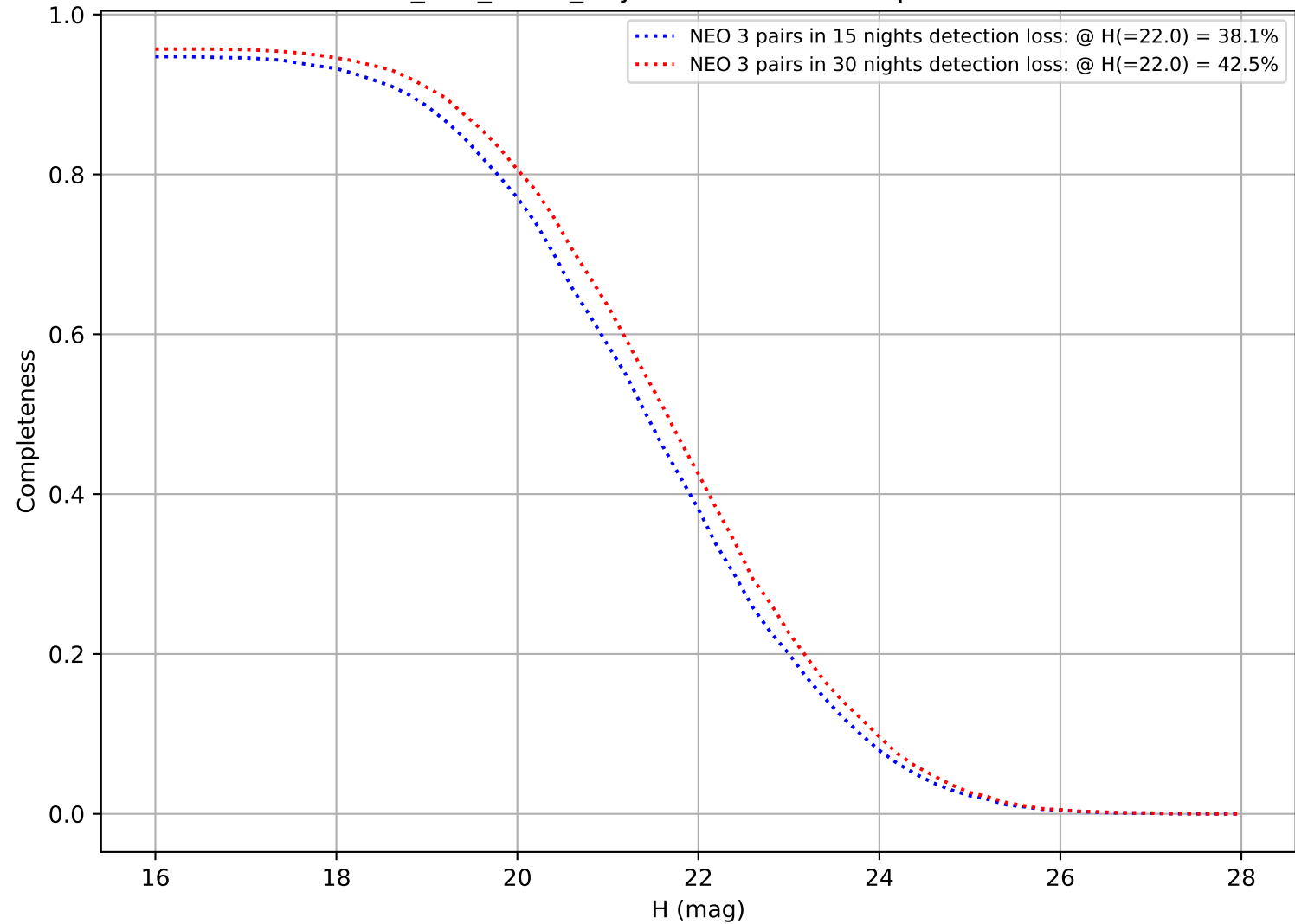
too_100_1v3.4_10yrs: DifferentialCompleteness
