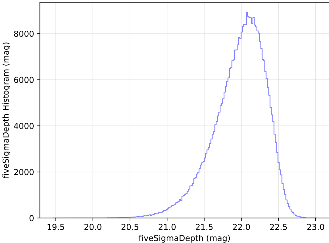
too_100_1v3.4_10yrs y: fiveSigmaDepth Histogram
