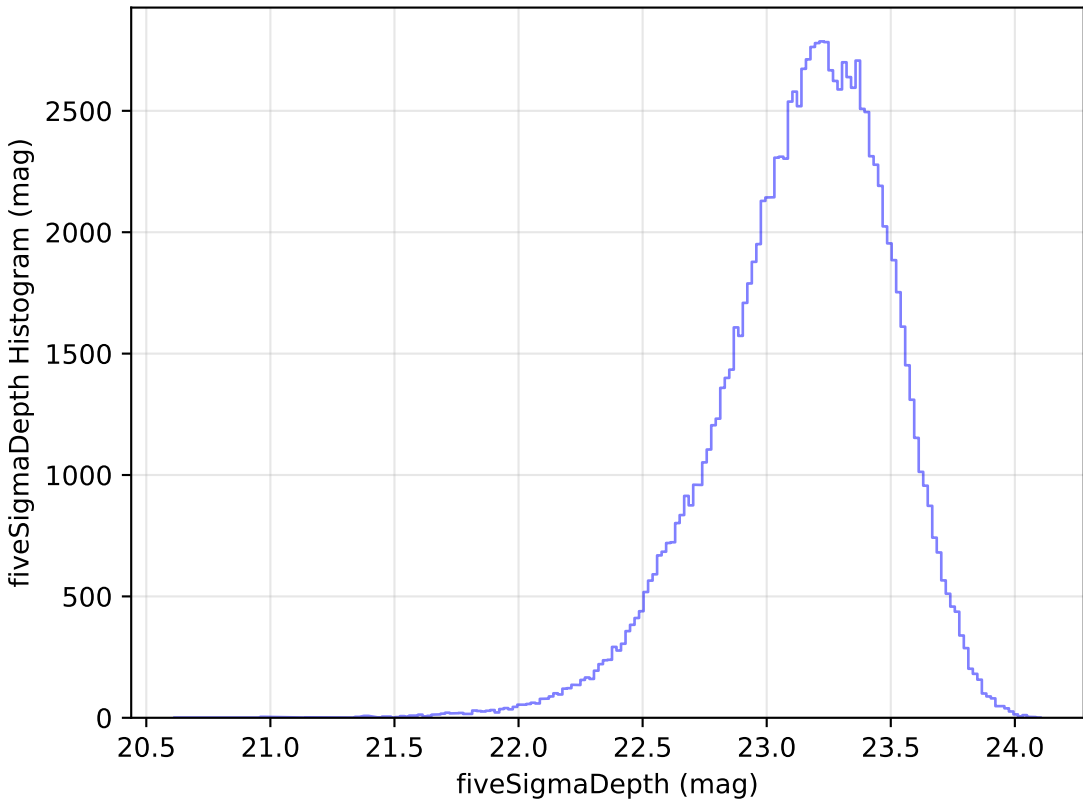
too_100_1v3.4_10yrs u: fiveSigmaDepth Histogram
