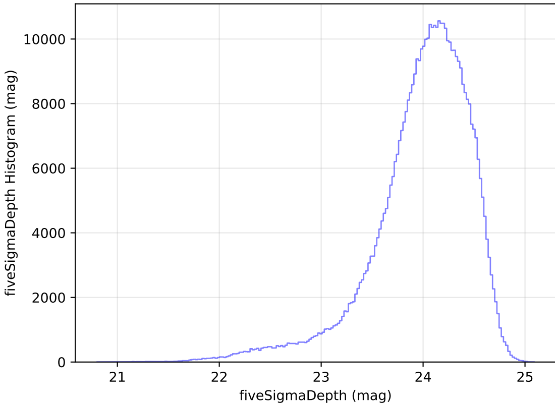
too_100_1v3.4_10yrs r: fiveSigmaDepth Histogram
