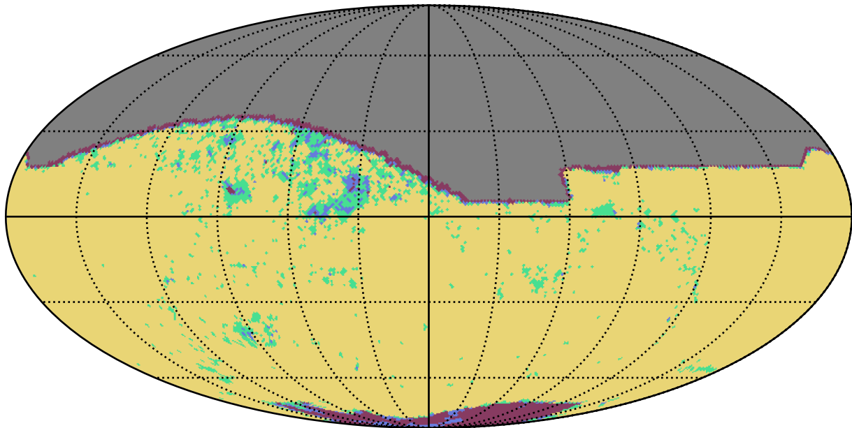
too_100_1v3.4_10yrs z band: YearCoverage night
