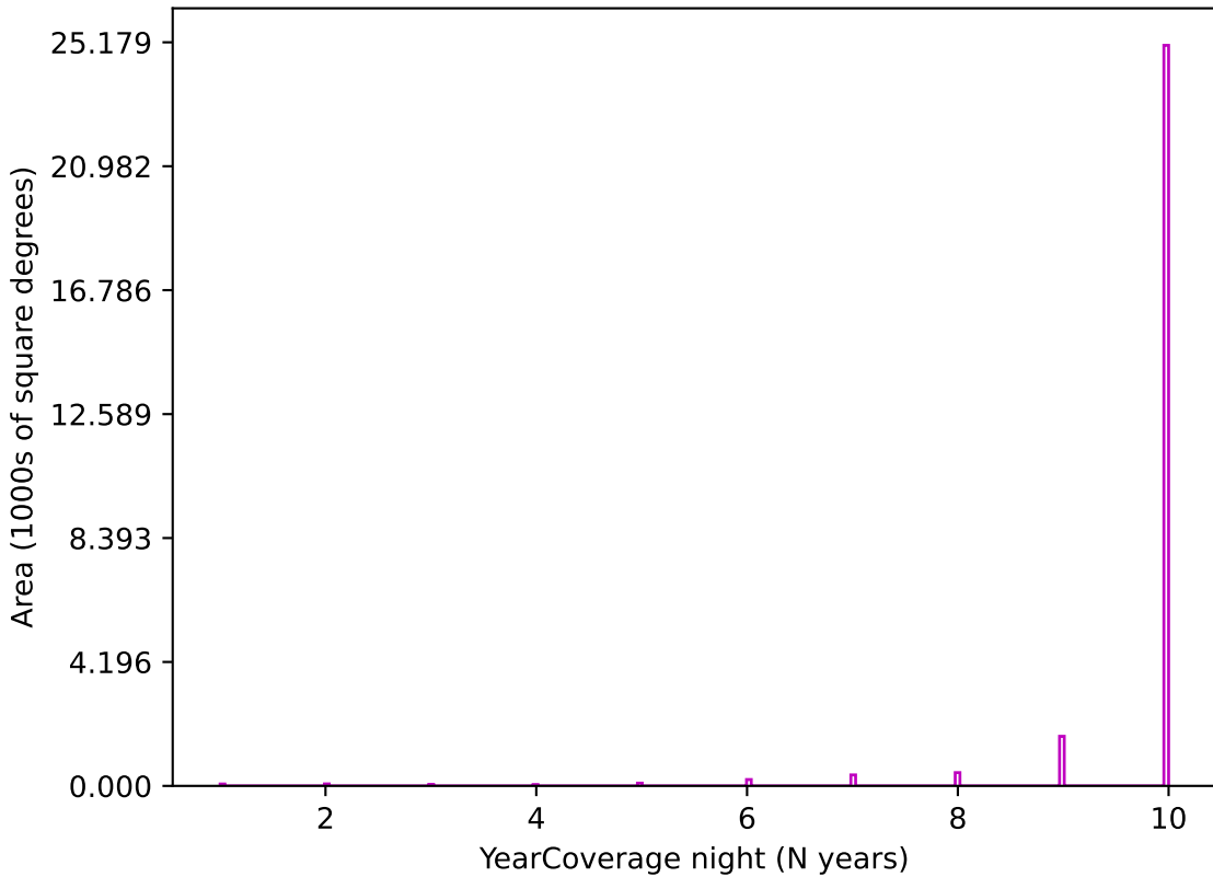
too_100_1v3.4_10yrs z band: YearCoverage night
