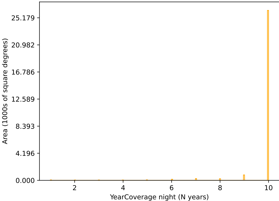
too_100_1v3.4_10yrs r band: YearCoverage night
