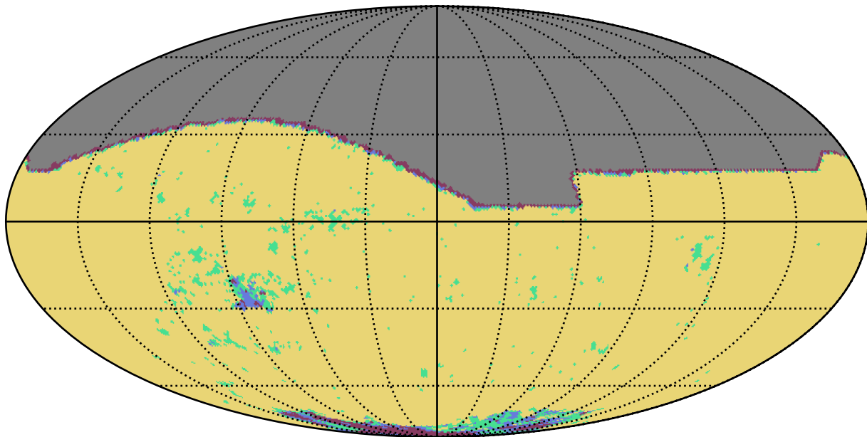
too_100_1v3.4_10yrs i band: YearCoverage night
