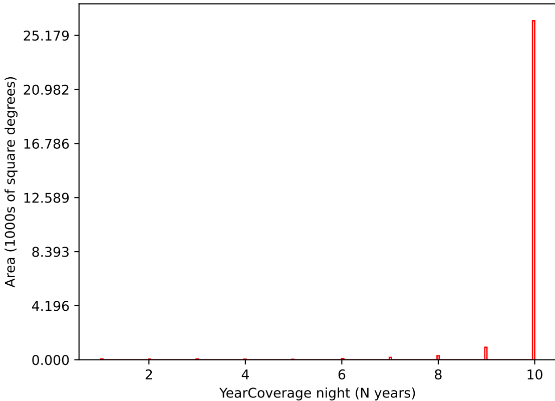
too_100_1v3.4_10yrs i band: YearCoverage night
