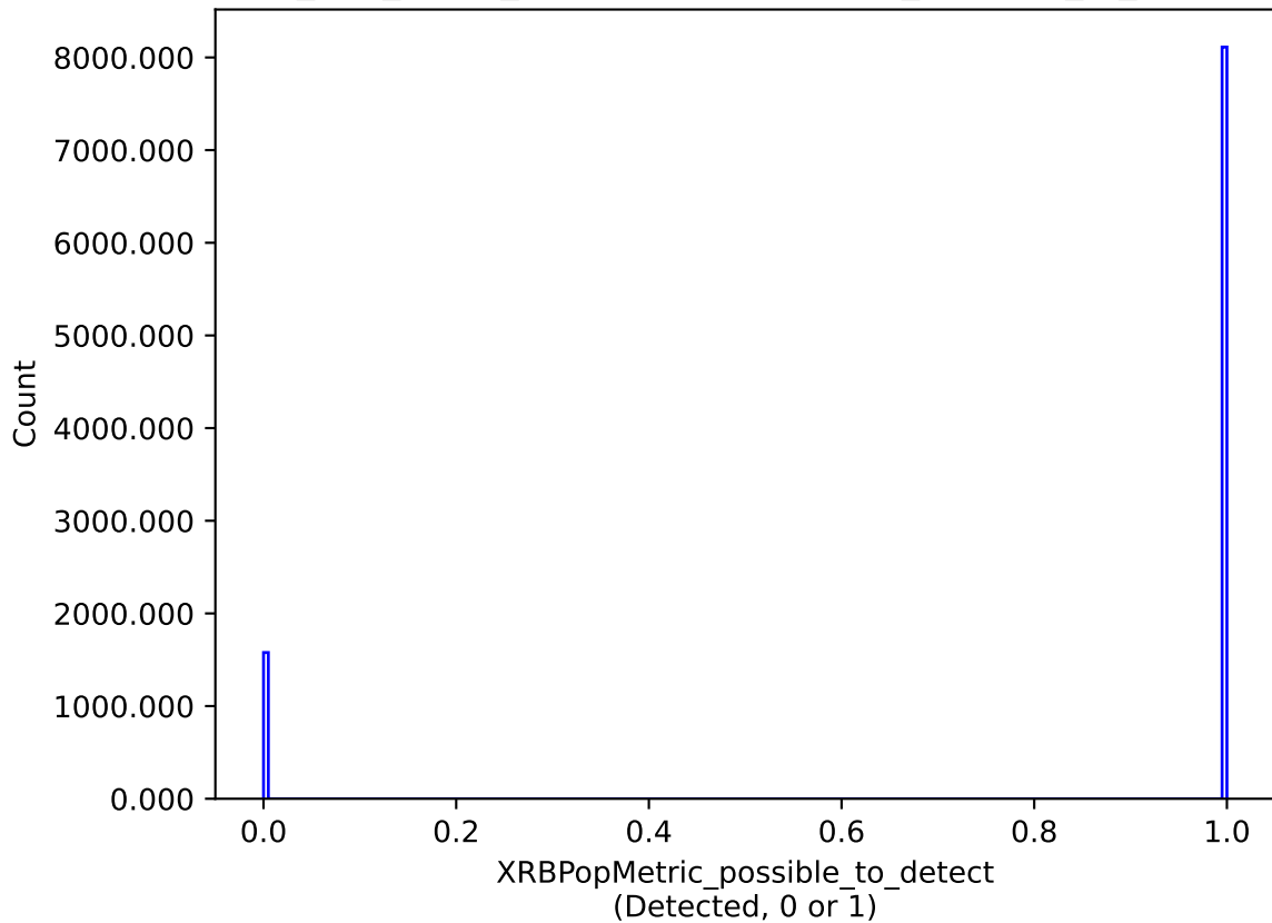
too_100_1v3.4_10yrs : XRBPoMetric_possible_to_detect
