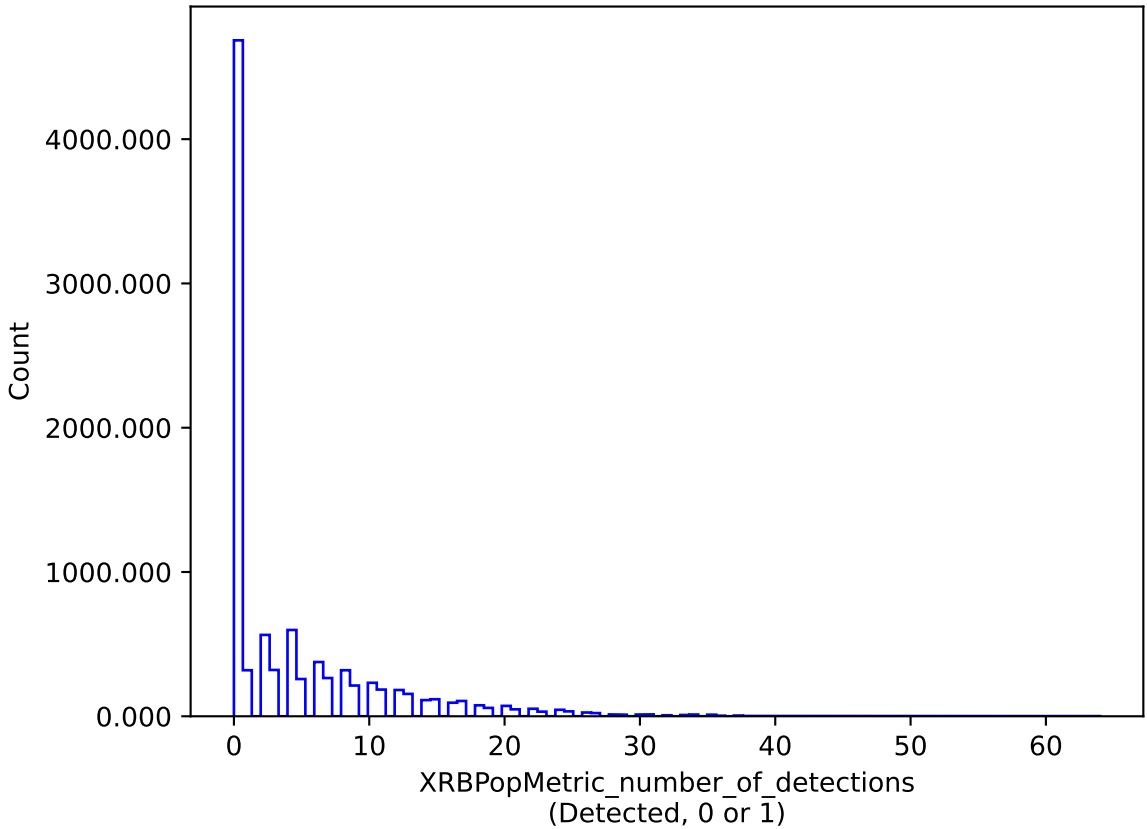
too_100_1v3.4_10yrs : XRBPoMetric_number_of_detections
