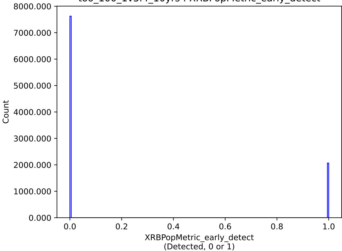
too_100_1v3.4_10yrs : XRBPoMetric_early_detect
