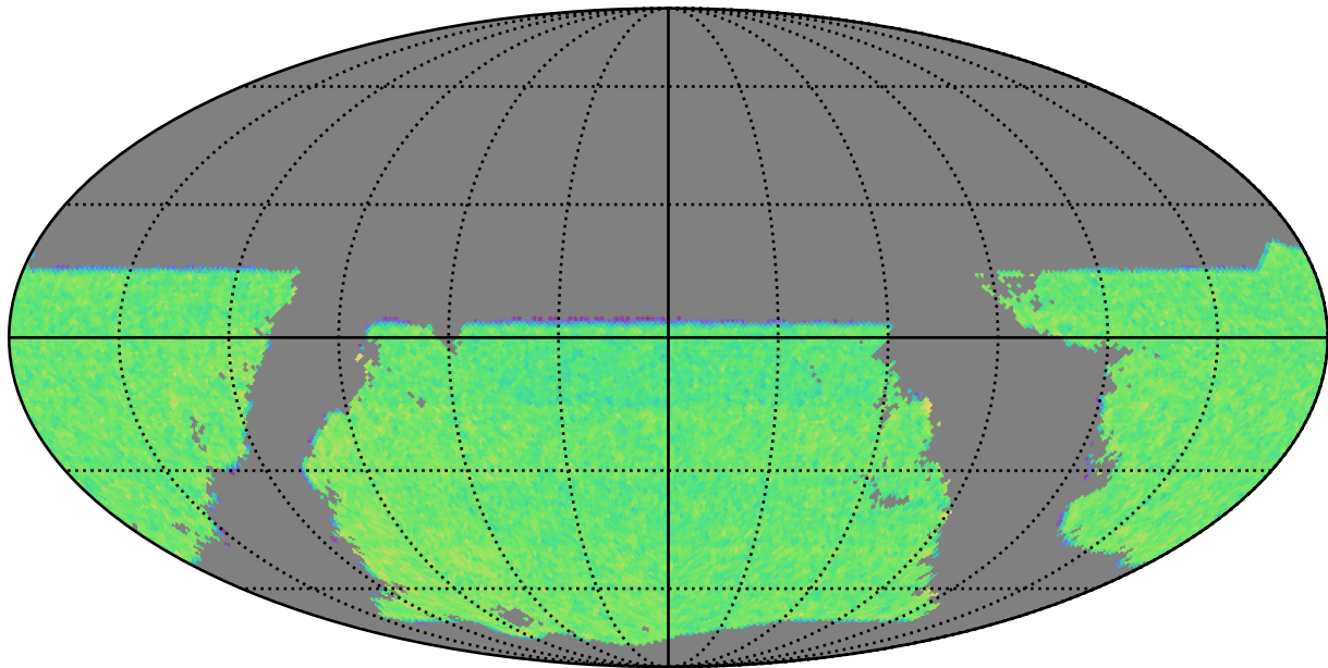
too_100_1v3.4_10yrs gri band non-DD: WeakLensingNvisits
