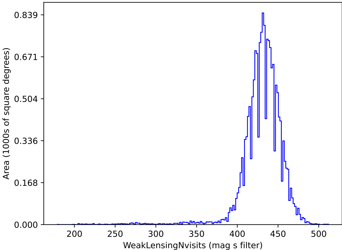
too_100_1v3.4_10yrs gri band non-DD: WeakLensingNvisits
