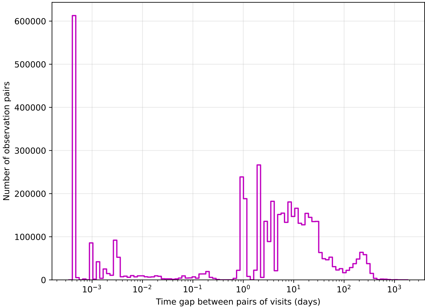
too_100_1v3.4_10yrs z band: Tgaps observationStartMJD
