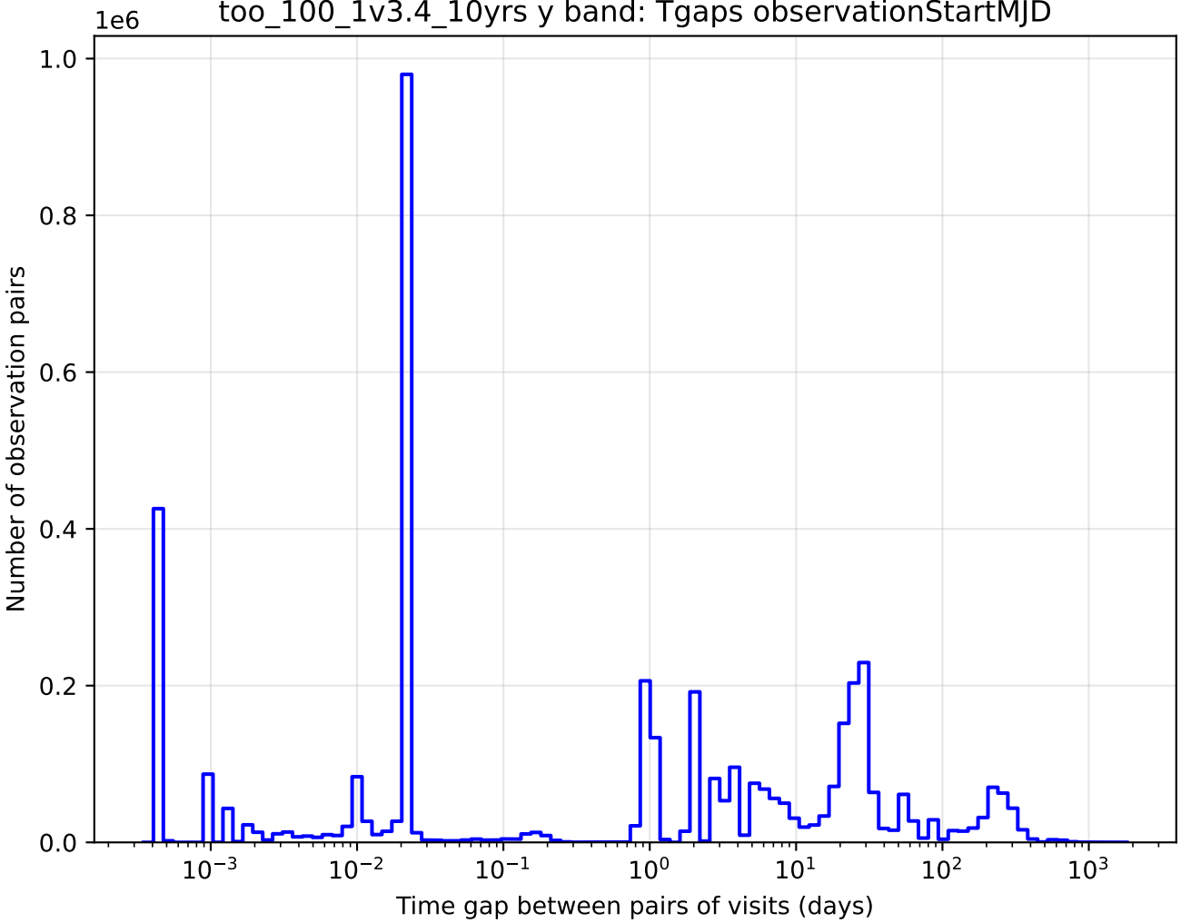
too_100_1v3.4_10yrs y band: Tgaps observationStartMJD
