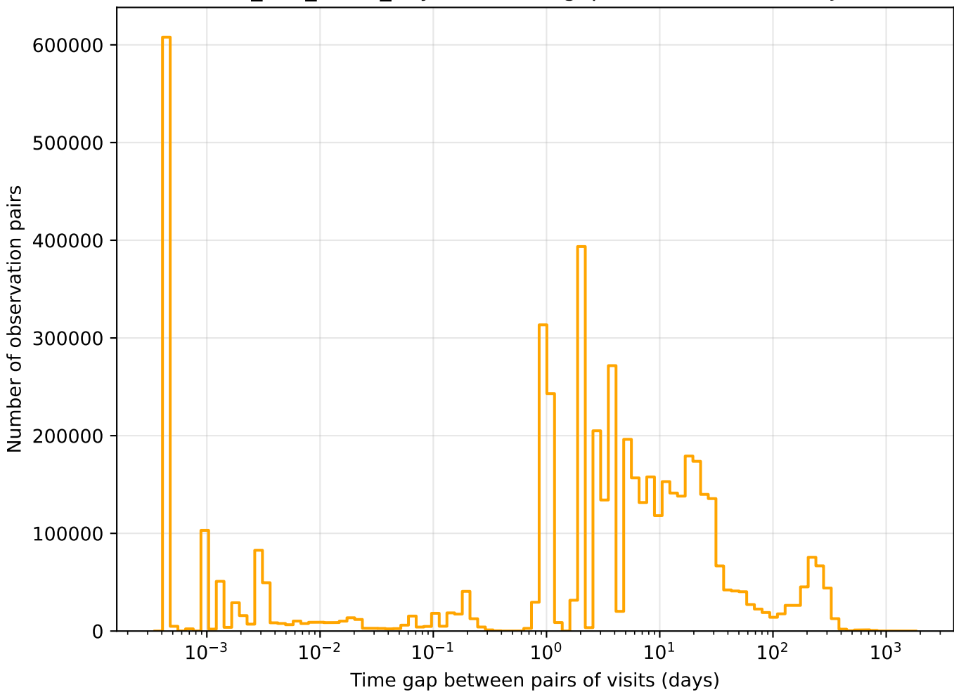
too_100_1v3.4_10yrs r band: Tgaps observationStartMJD
