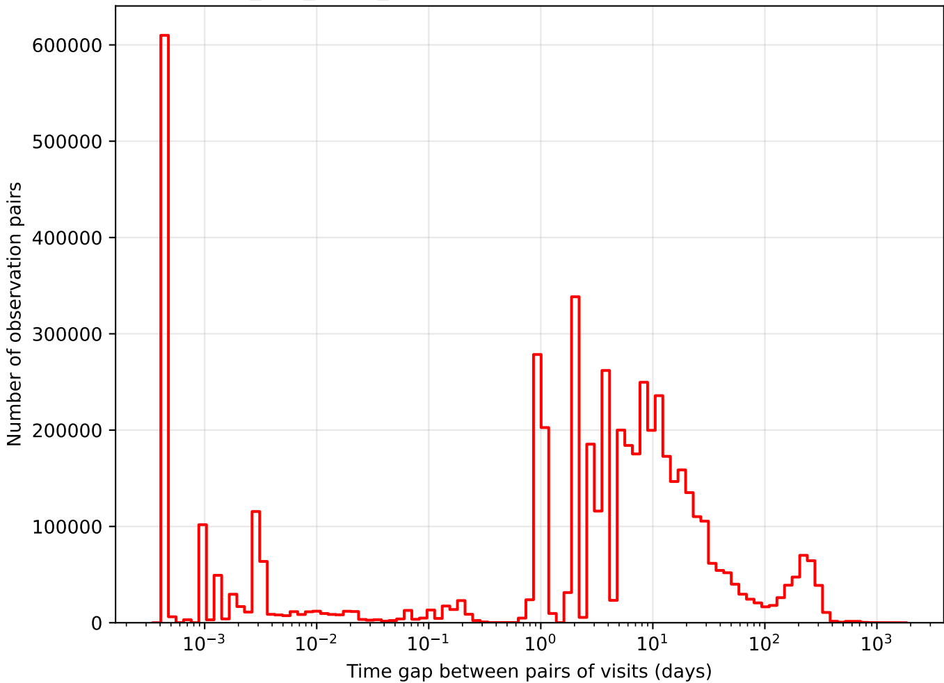
too_100_1v3.4_10yrs i band: Tgaps observationStartMJD
