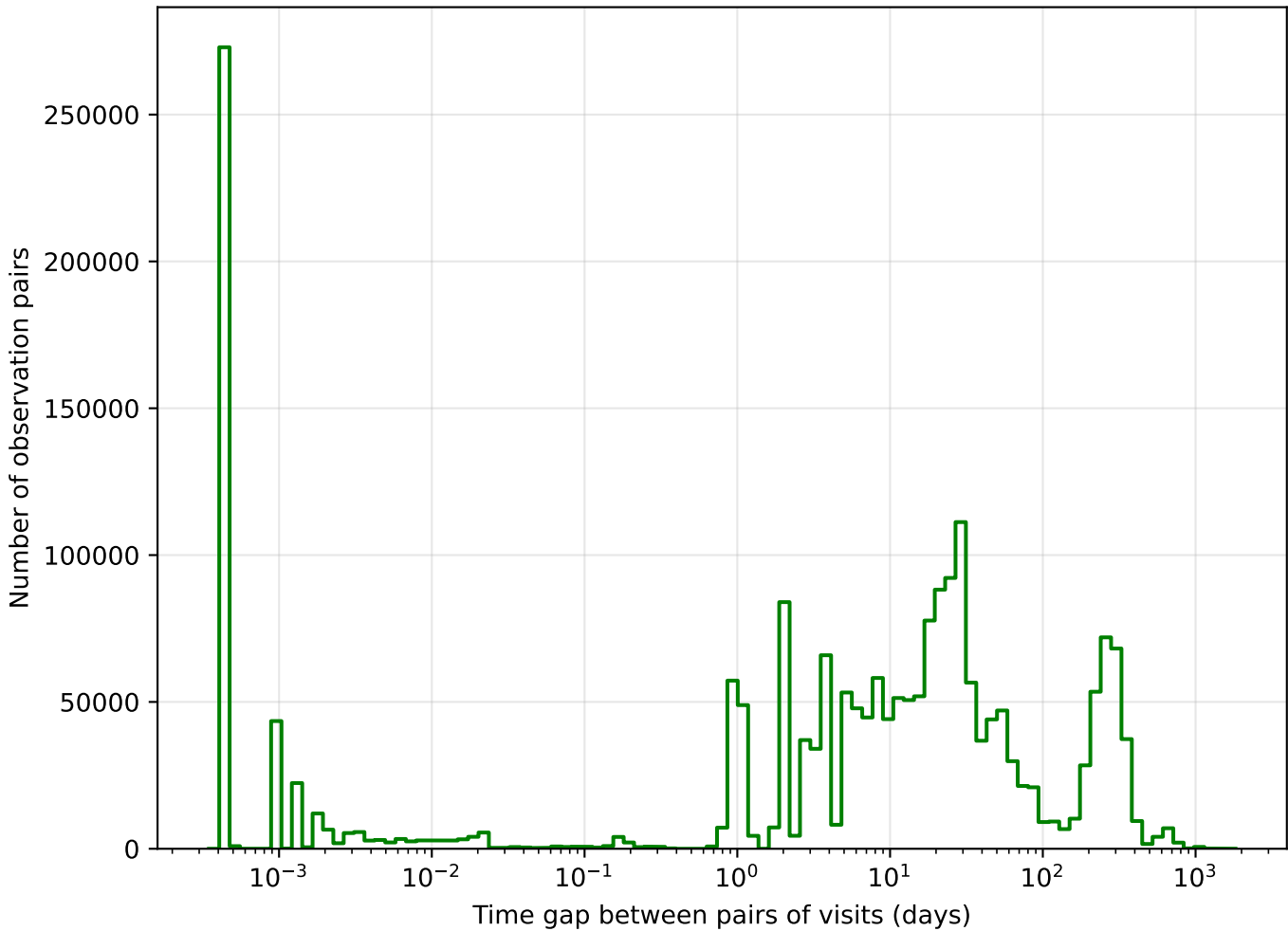
too_100_1v3.4_10yrs g band: Tgaps observationStartMJD
