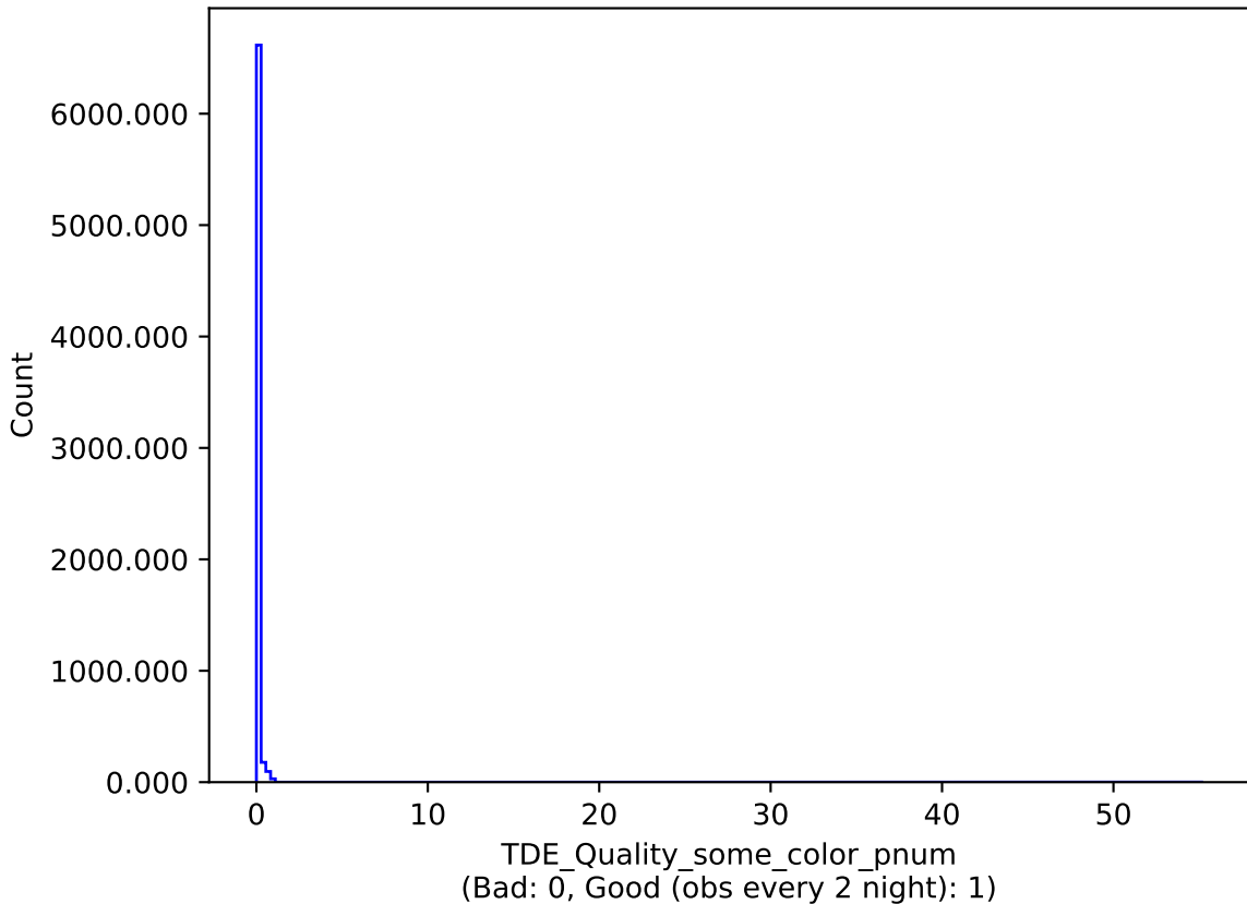
too_100_1v3.4_10yrs : TDE_Quality_some_color_pnum
