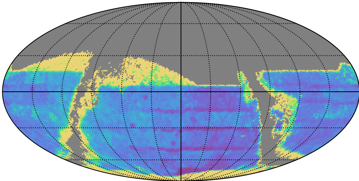
too_100_1v3.4_10yrs : TDC_accuracy
