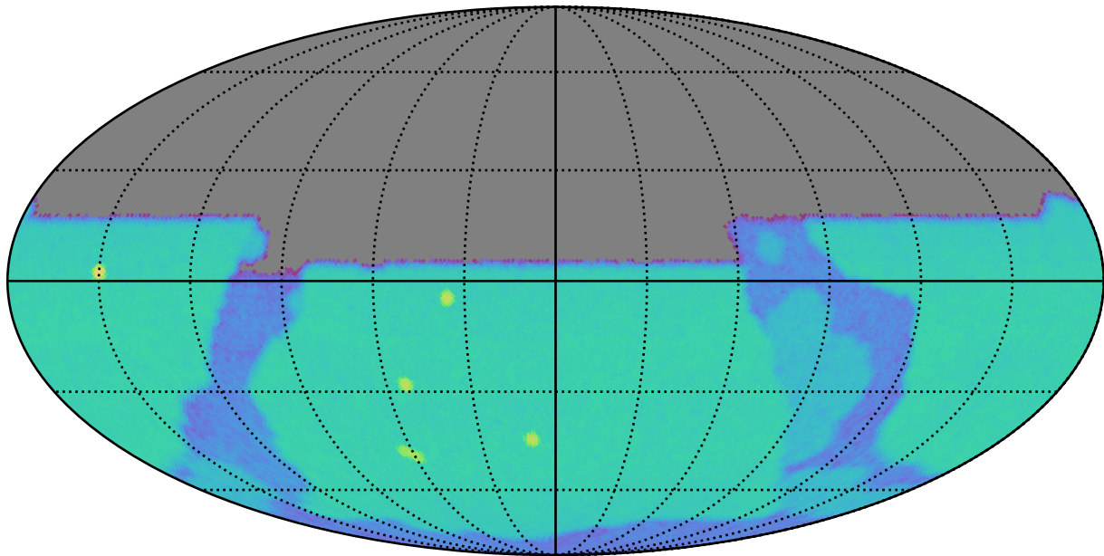
too_100_1v3.4_10yrs u: SurfaceBrightLimit
