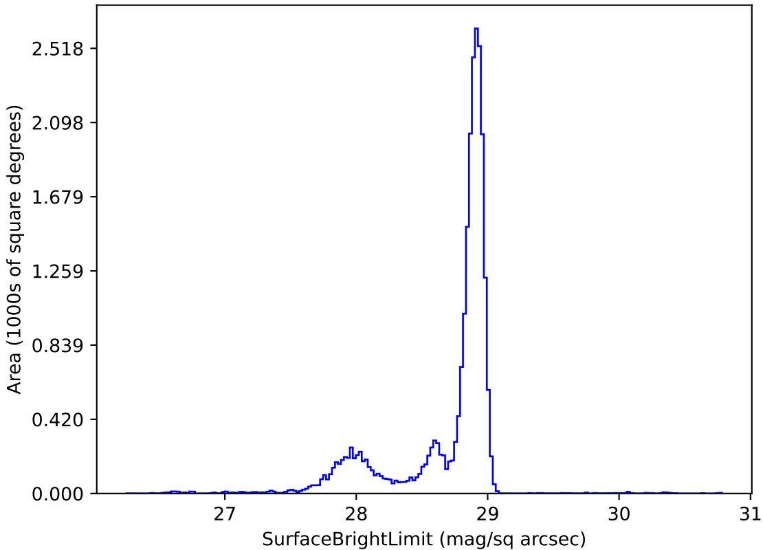
too_100_1v3.4_10yrs u: SurfaceBrightLimit
