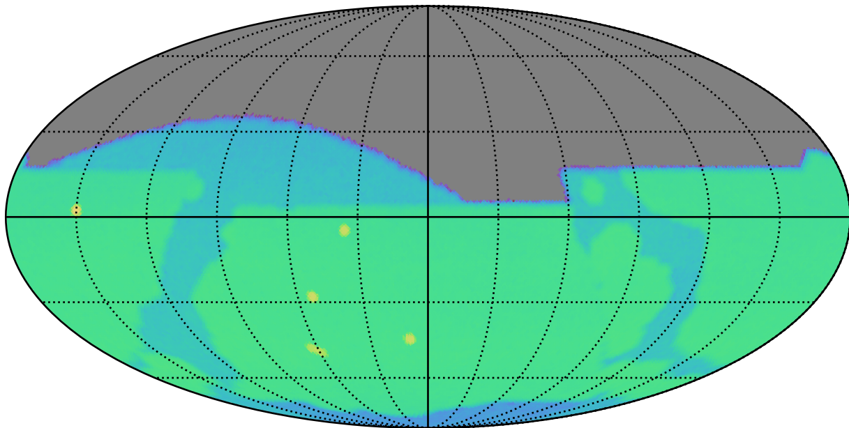
too_100_1v3.4_10yrs r: SurfaceBrightLimit
