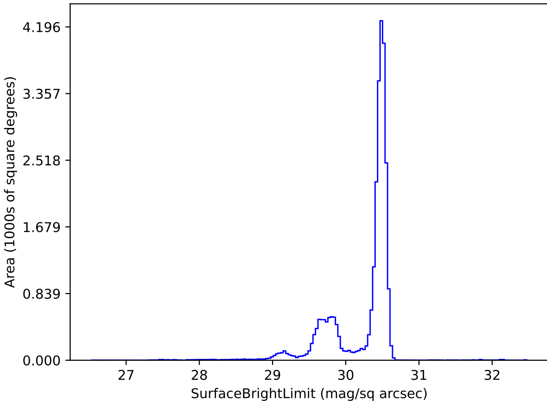
too_100_1v3.4_10yrs r: SurfaceBrightLimit
