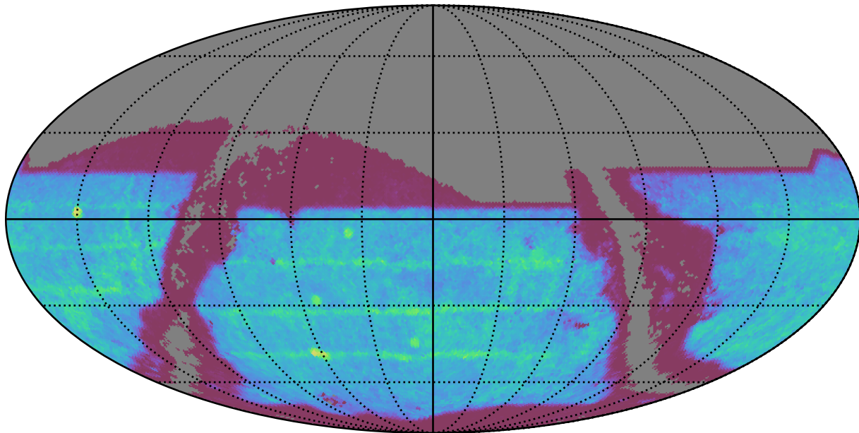
too_100_1v3.4_10yrs : SNSLMetric
