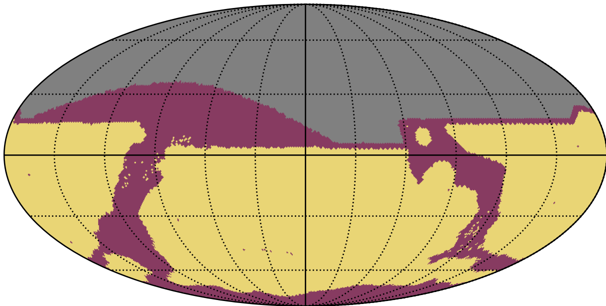
too_100_1v3.4_10yrs : RapidRevisits
