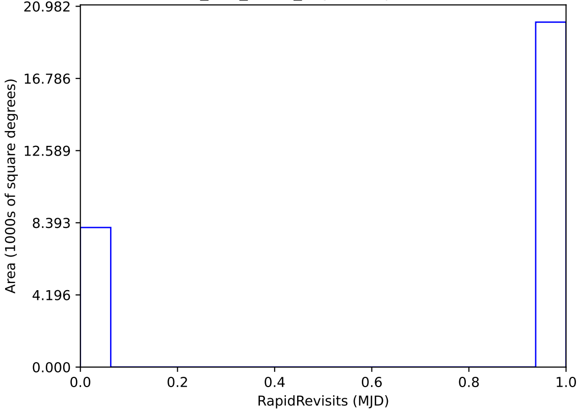
too_100_1v3.4_10yrs : RapidRevisits
