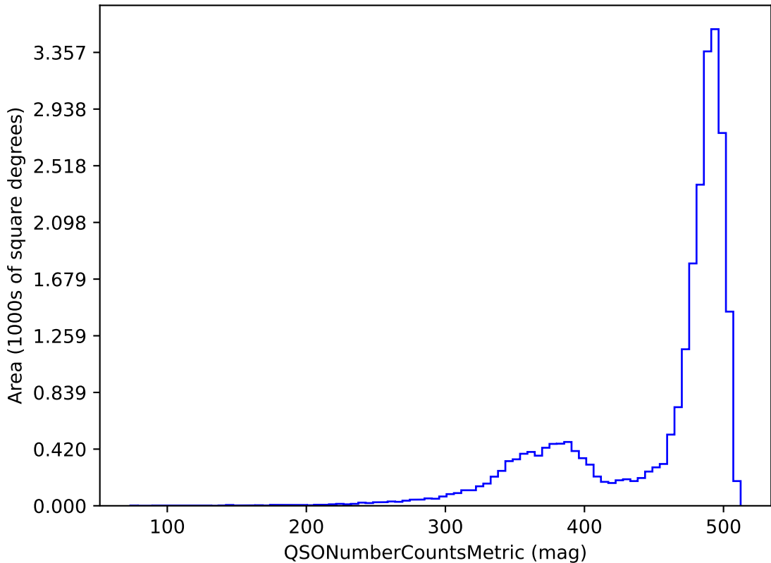
too_100_1v3.4_10yrs z band and non-DD: QSONumberCountsMetric
