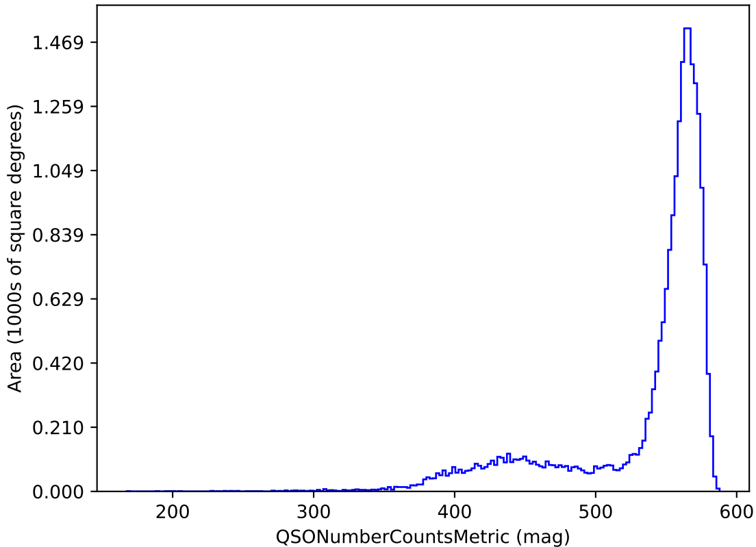
too_100_1v3.4_10yrs y band and non-DD: QSONumberCountsMetric
