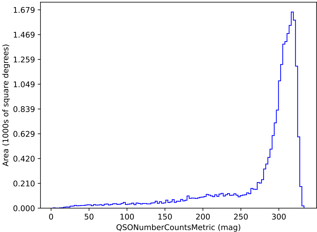
too_100_1v3.4_10yrs u band and non-DD: QSONumberCountsMetric
