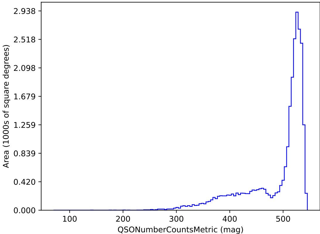
too_100_1v3.4_10yrs r band and non-DD: QSONumberCountsMetric
