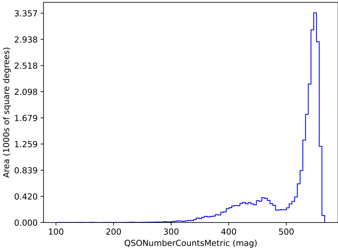
too_100_1v3.4_10yrs i band and non-DD: QSONumberCountsMetric
